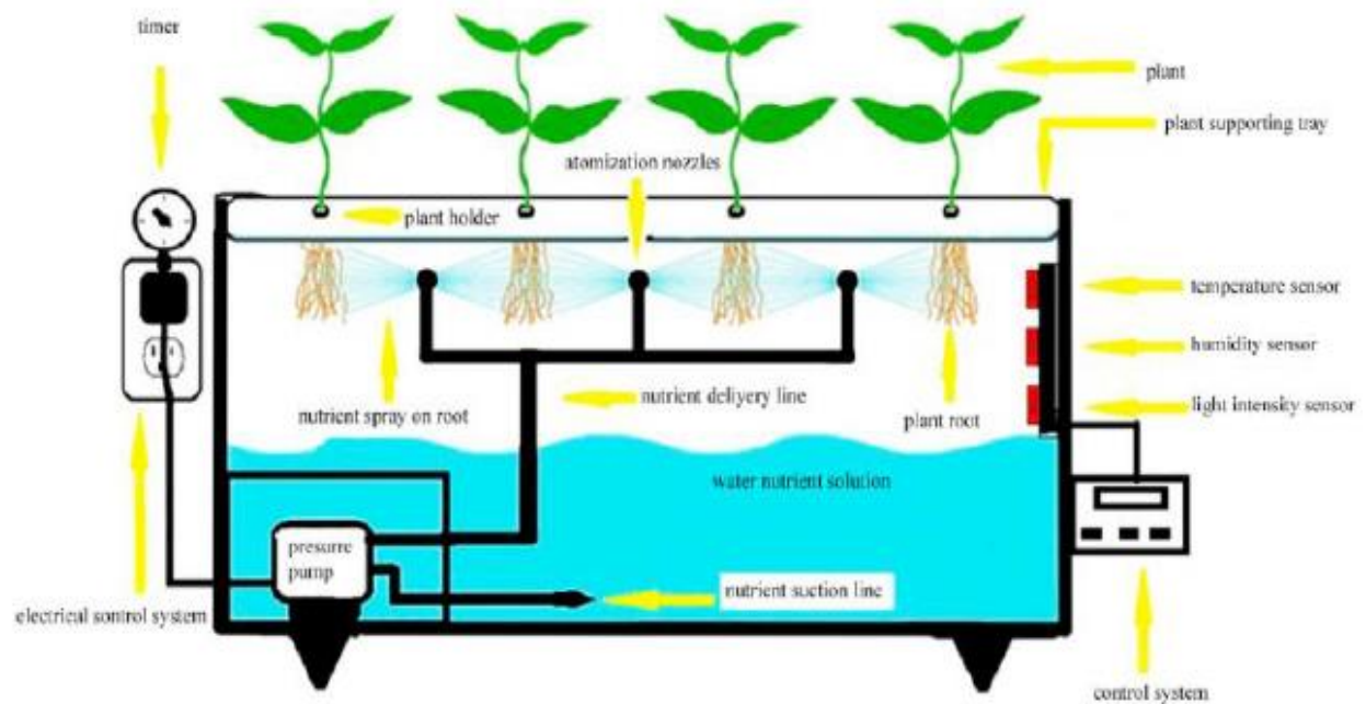
Figure : Aeroponics Misting System
