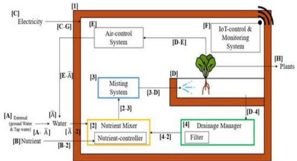
Figure : Aeroponics Smart Farm
